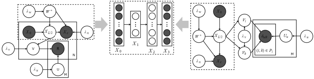
Fig. 5. Graphical model of collaborative deep learning (left) and collaborative deep ranking (right).
