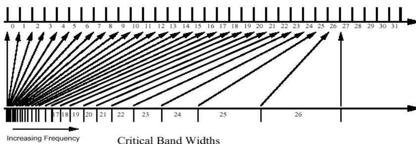
MPEG/Audio Filter Bank Bands
