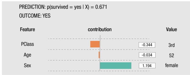
Fig. 3. Example of linear model and the returned features importance.
