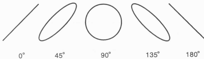
(b) LISSAJOUS PATTERNS OF VARIOUS PHASE ANGLES
