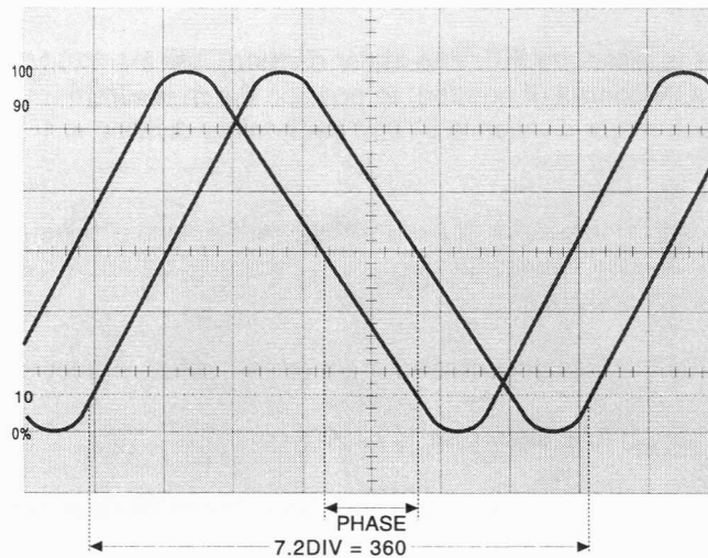
Figure 2-11: Dual-Trace Method of Phase Measurement
