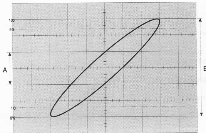
(a) PHASE ANGLE CALCULATION
